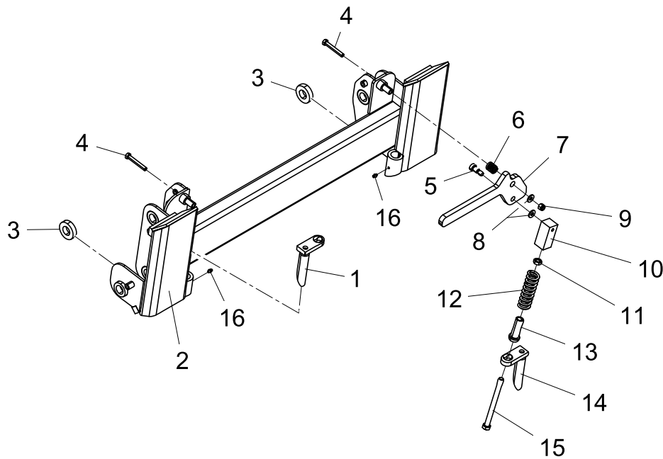
2014-397 Quick Attach Assembly (includes all items shown)
