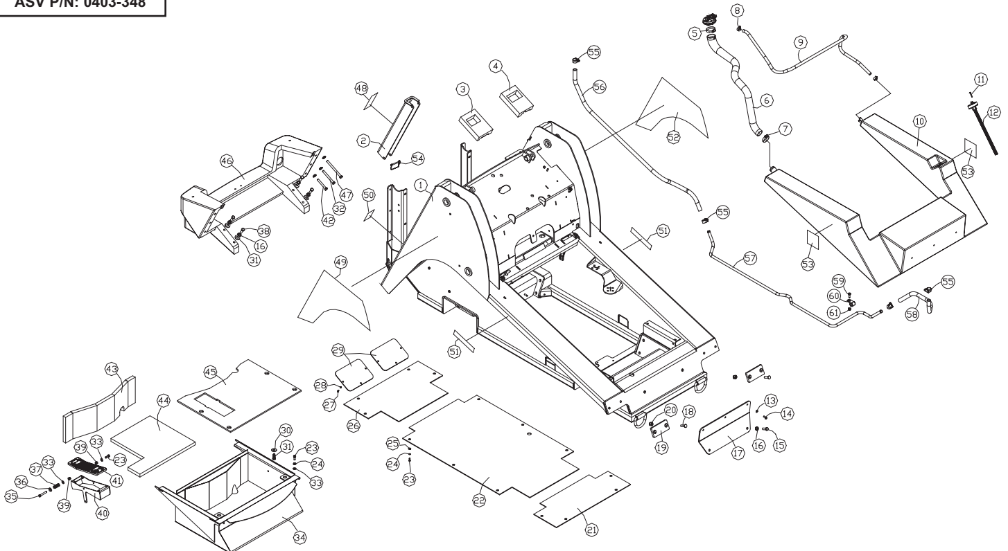
RH Fuel Tank Vent Kit ASV P/N: 0403-348
