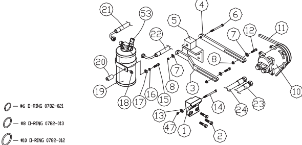
COMPRESSOR ASSEMBLY
