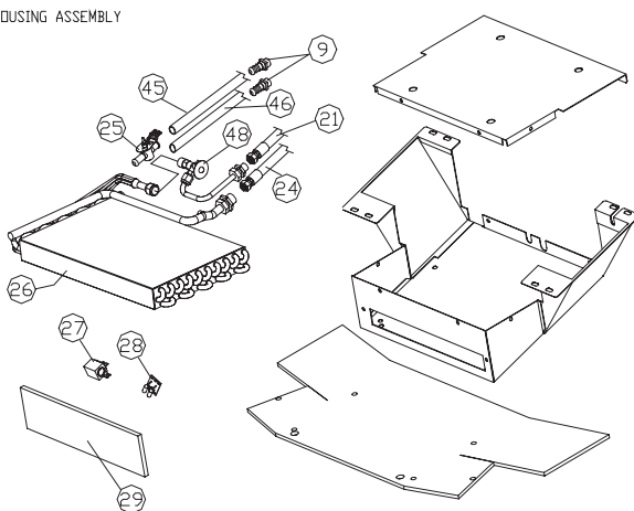
LOWER HOUSING ASSEMBLY
