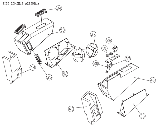
SIDE CONSOLE ASSEMBLY
