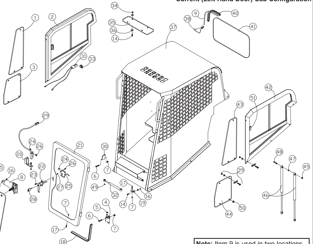
Current (Left Hand Door) Cab Configuration
