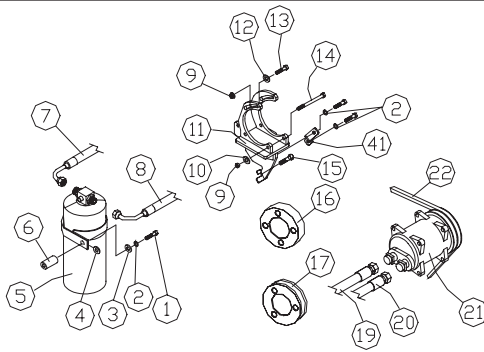
COMPRESSOR ASSEMBLY
