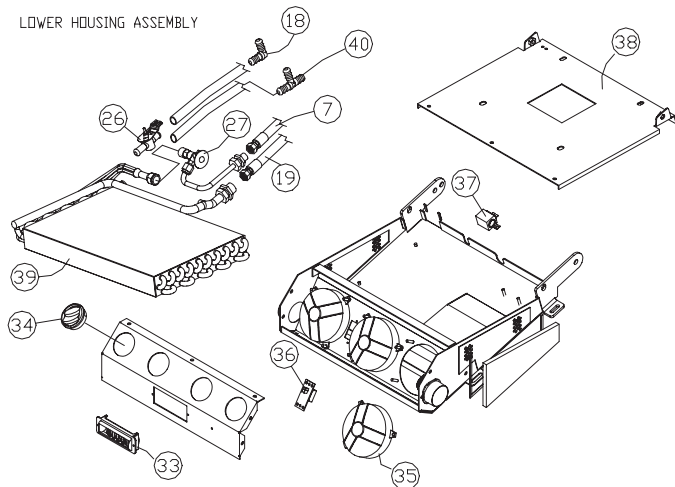
LOWER HOUSING ASSEMBLY
