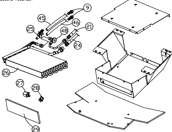
LOWER HOUSING ASSEMBLY
