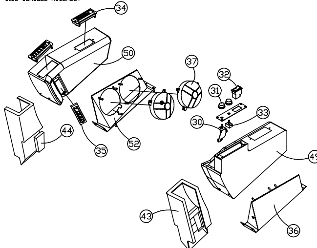
SIDE CONSOLE ASSEMBLY
