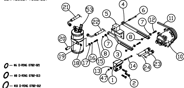
COMPRESSOR ASSEMBLY
