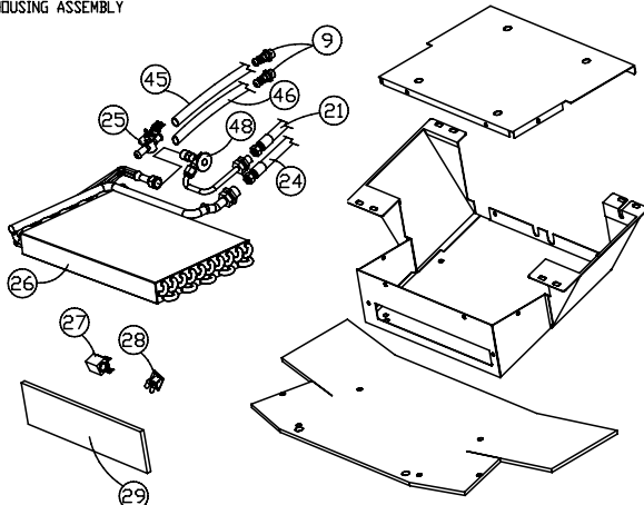
LOWER HOUSING ASSEMBLY
