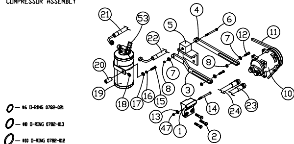
COMPRESSOR ASSEMBLY
