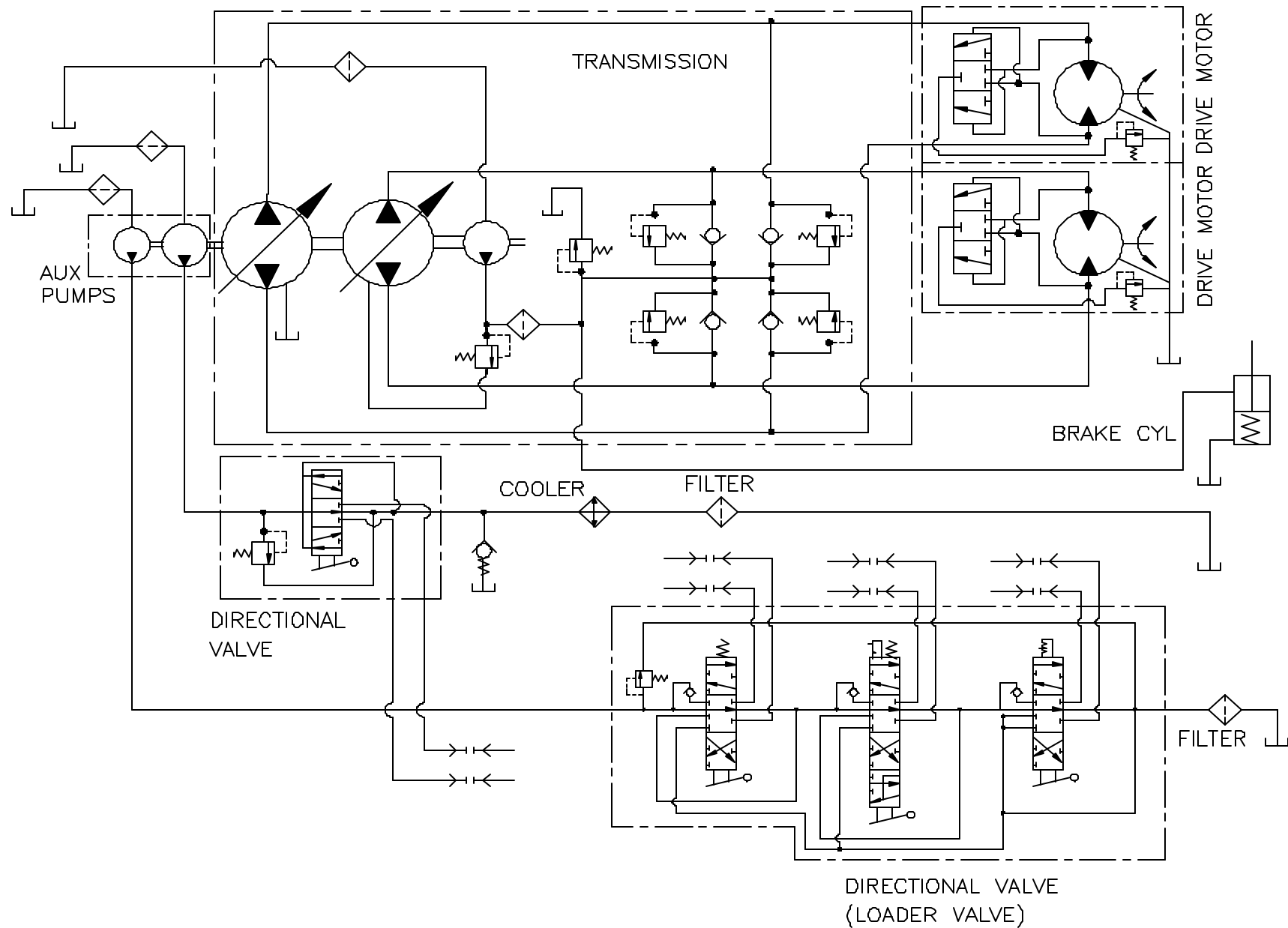
HYDRAULIC SCHEMATIC MD2800/MD2810
