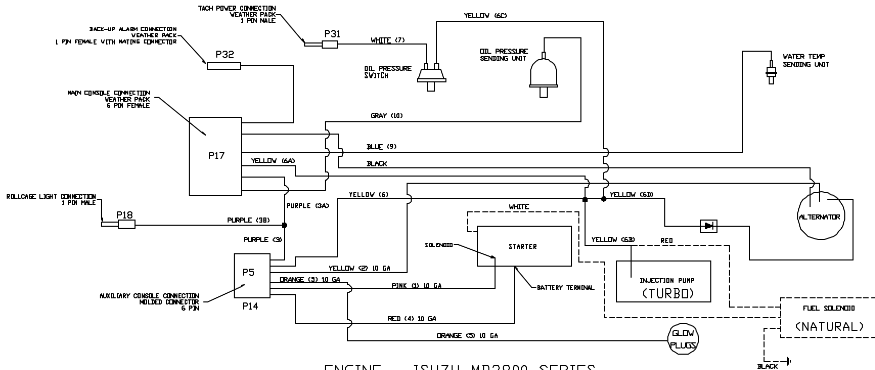
ENGINE - ISUZU MD2800 SERIES
