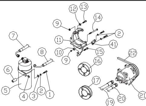
COMPRESSOR ASSEMBLY
