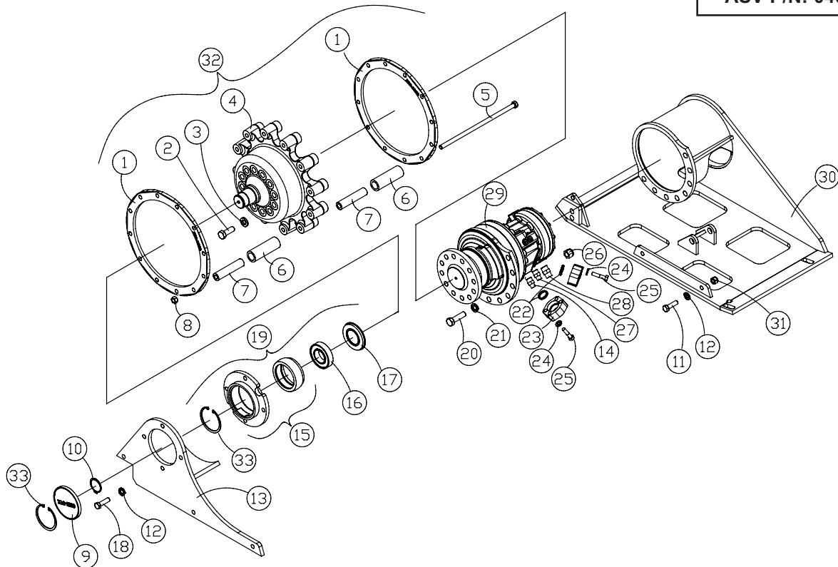
Drive Motor Seal Kit ASV P/N: 0403-871
