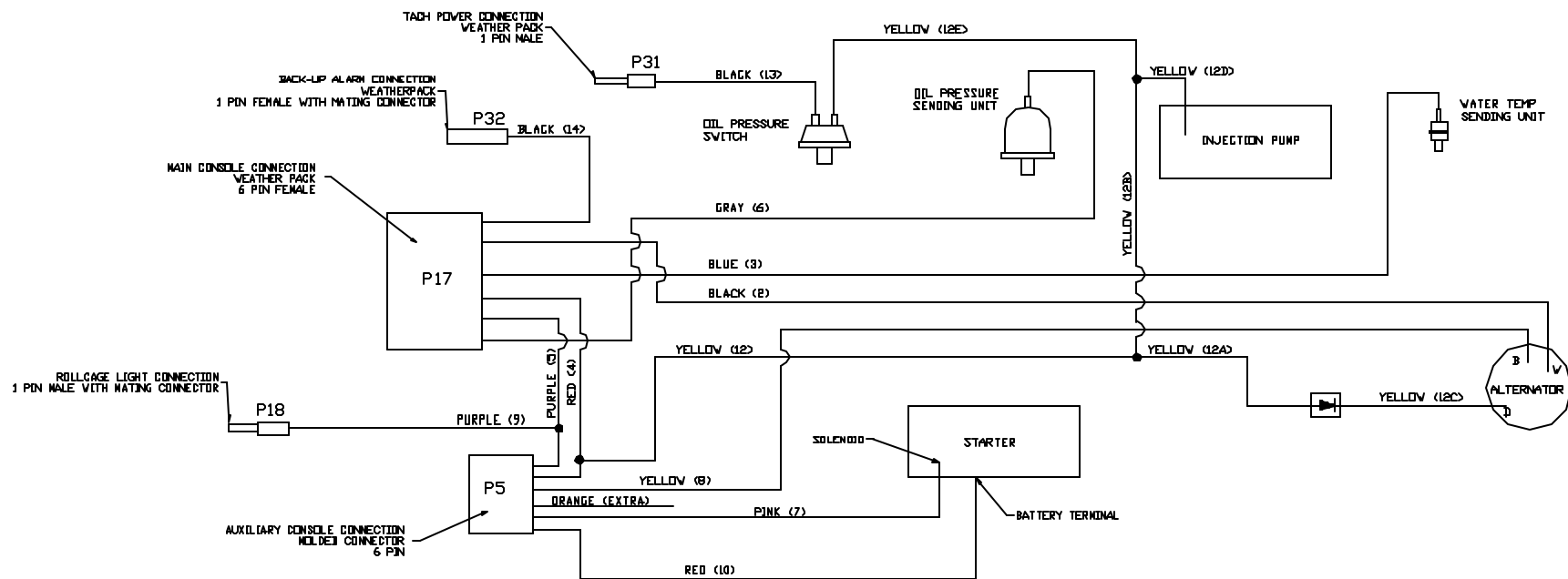
JOHN DEERE 4045 ENGINE
